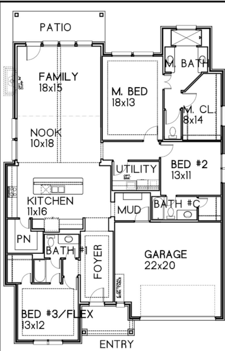
FLOOR PLAN - FIRST "2332A" LOTS 2-11 2,334 S.F.
