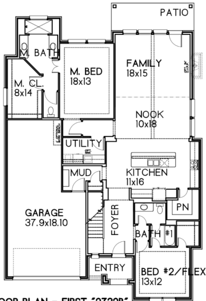
FLOOR PLAN - FIRST "2732B" LOTS 2-11 2,734 S.F.
