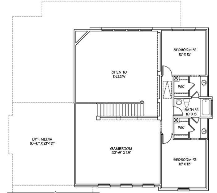
SECOND FLOOR PLAN-A 1035 SQ. FT.
