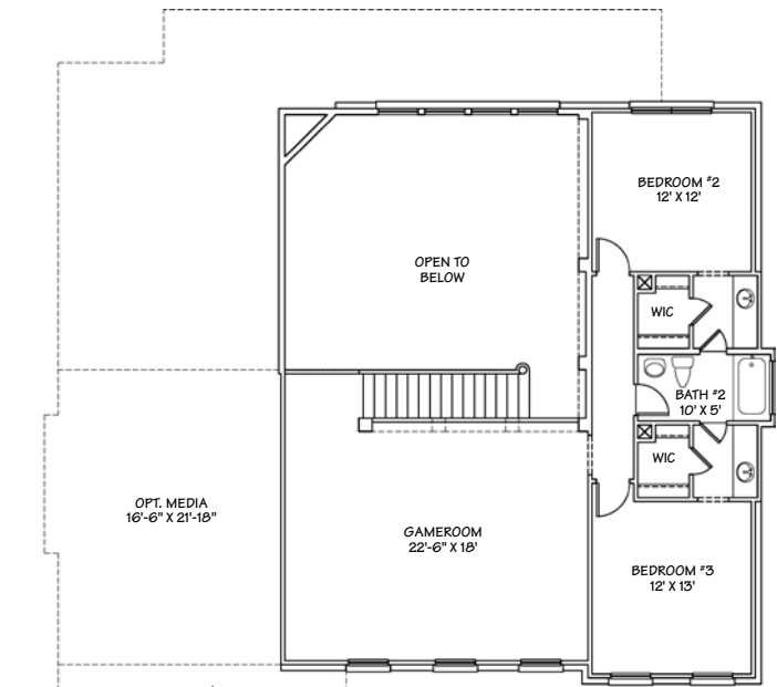
SECOND FLOOR PLAN-B 1035 SQ. FT.
