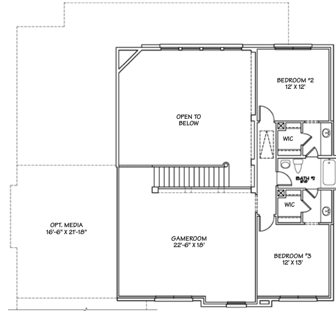
SECOND FLOOR PLAN-C 1033 SQ. FT.
